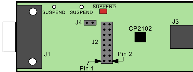
Figure 2. CP2102 Evaluation Board
