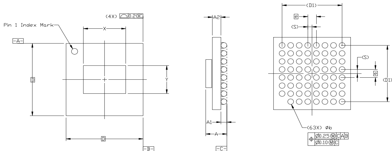
Figure 12. 63-Ball Ceramic Ball Grid Array (CBGA)
